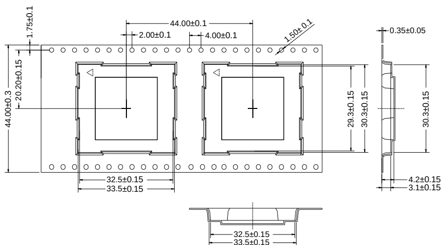
Figure 51: Tape Specifications
