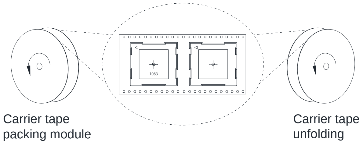
Figure 53: Tape and Reel Directions
