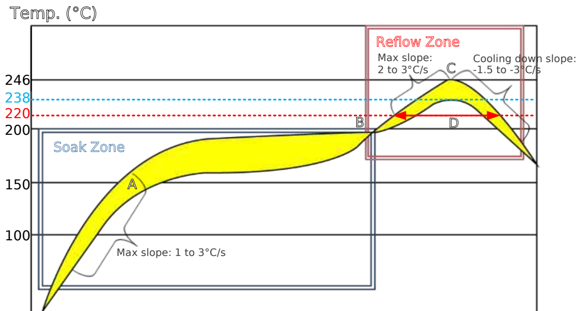
Figure 50: Reflow Soldering Thermal Profile
