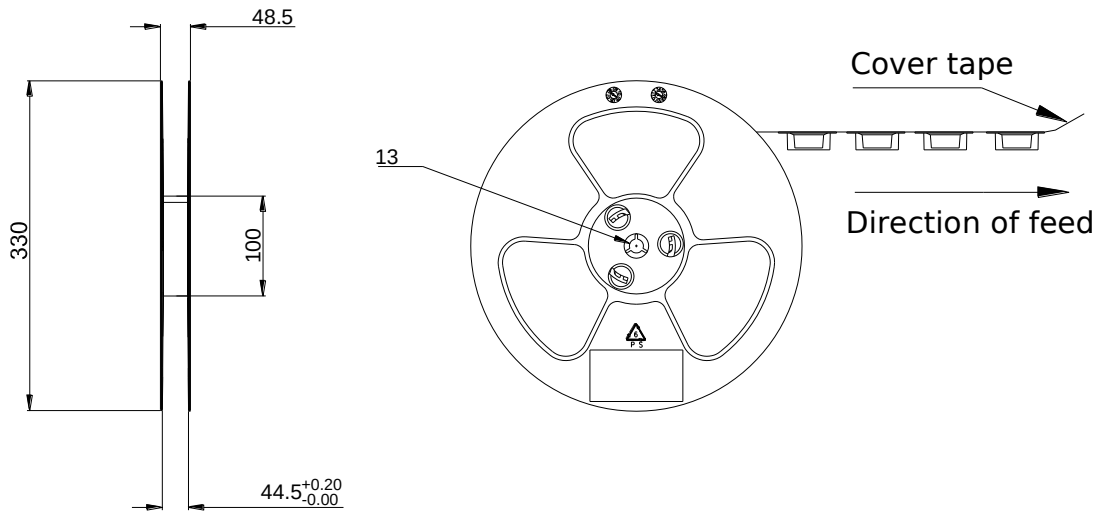
Figure 52: Reel Specifications
